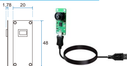
B2020U-6B Board type / Up view / 6B Lens
