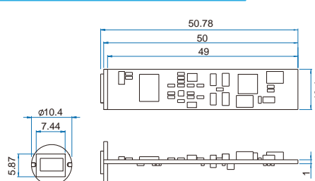
B2011 Board type / Front view / No Lens
