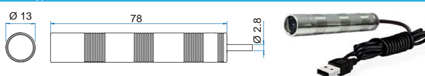
T2013 Tube type / Front View / 3.0mm F 2.0 Lens
