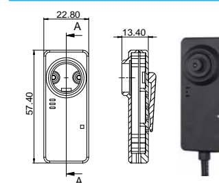
N2020U Case type / Up view / Built-In Lens
